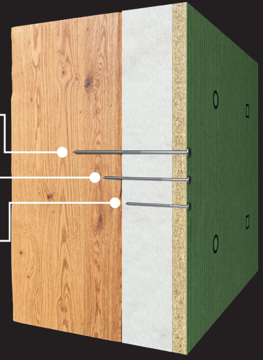
ZIP System® R-Sheathing (Factory-laminated)
